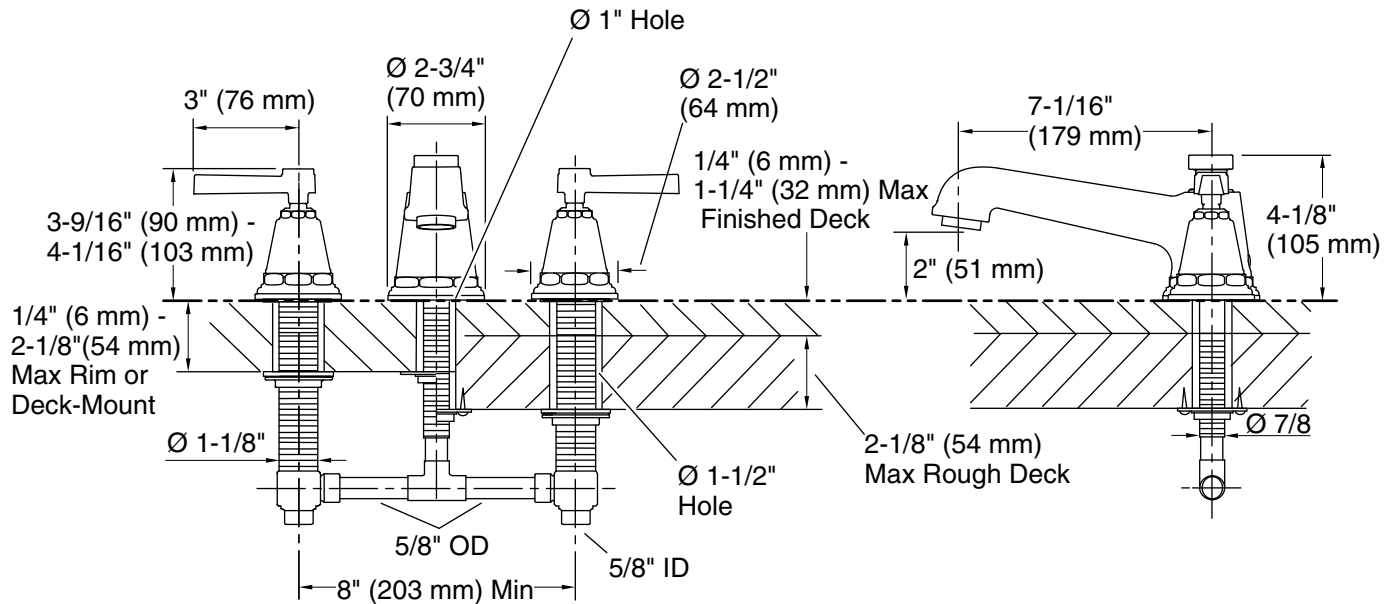
Rough + Finished Deck-Mount Installation
